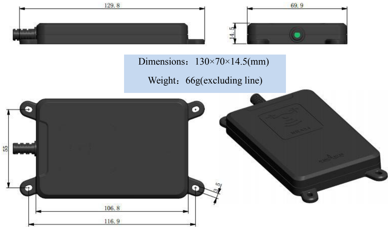
Figure 1 NRA24 outlook
